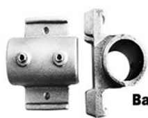
SMS166 1.66" Mounting Bracket Horizontal - Vertical
